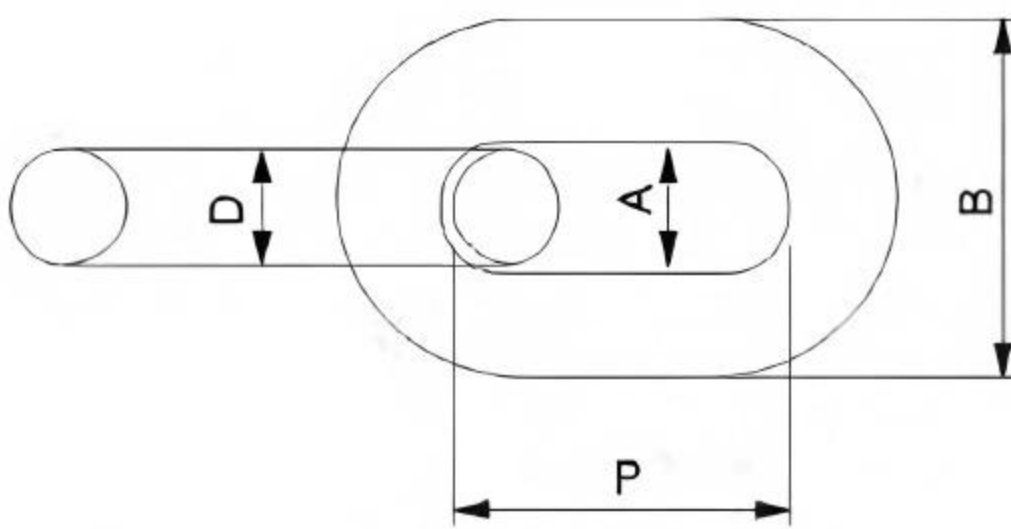
Chain 链条
